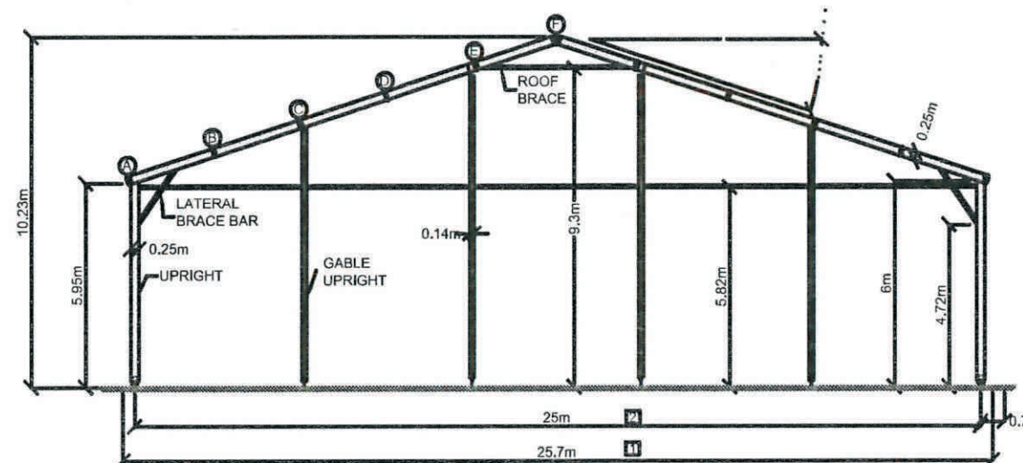
GABLE ELEVATION (SINGLE SKIN PVC ROOF & GABLES, STEEL CLADDING WALLS)
