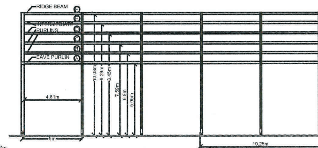
SIDE ELEVATION (SINGLE SKIN PVC ROOF & GABLES, STEEL CLADDING WALLS)
