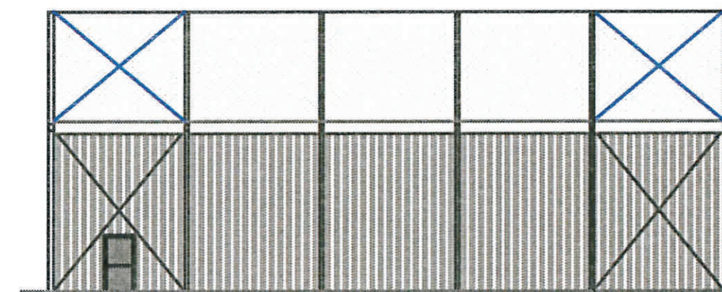
SIDE ELEVATION (SINGLE SKIN PVC ROOF & GABLES, STEEL CLADDING WALLS)
