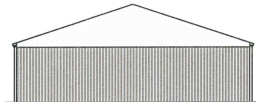
GABLE ELEVATION (SINGLE SKIN PVC ROOF & GABLES, STEEL CLADDING WALLS)
