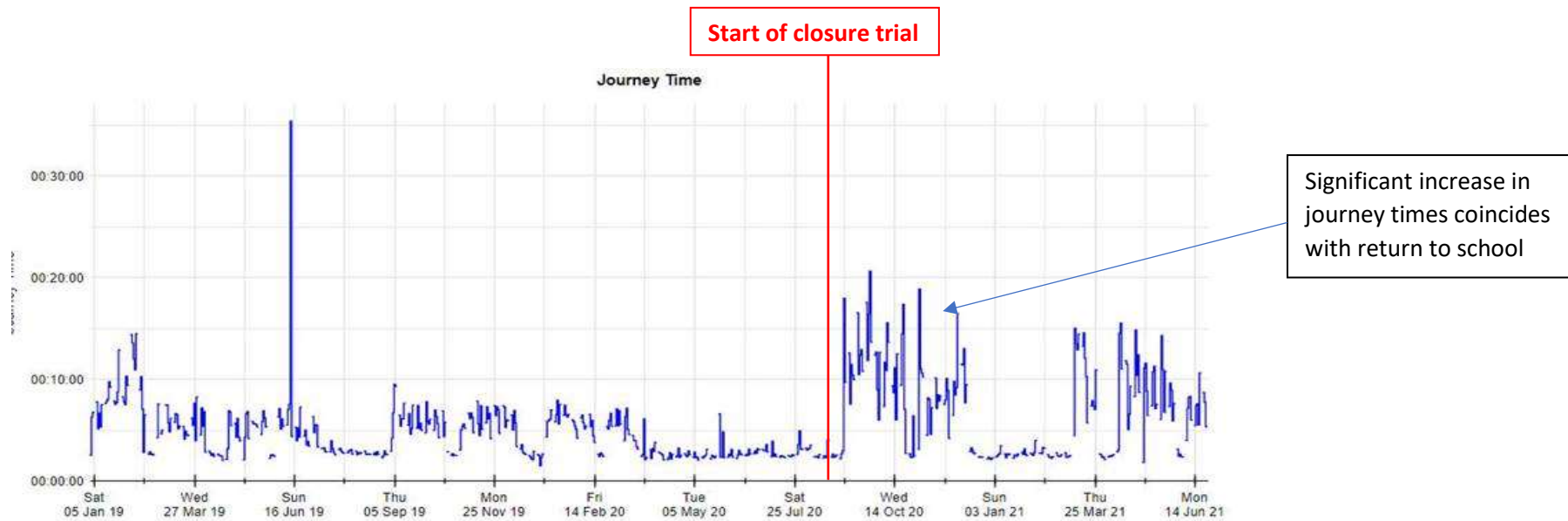
Long Road (eastbound) AM peak period journey times (based on blue tooth data)
